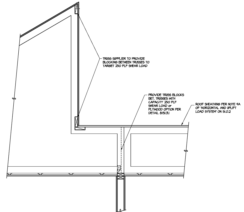
1 SECTION AT MECHANICAL WELLS NOT TO SCALE
