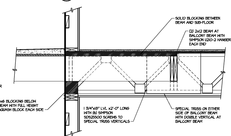
1 SECTION AT B6 BALCONY NOT TO SCALE
