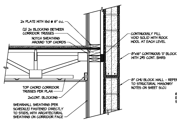
4 SECTION AT CORRIDOR NOT TO SCALE
