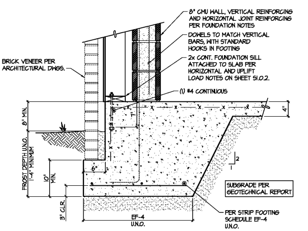
4 EXTERIOR FOOTING AT MASONRY WALL NOT TO SCALE
