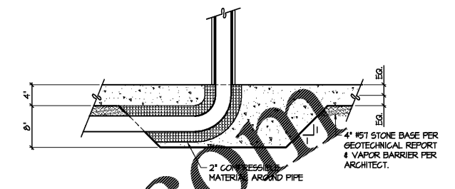
3 SECTION AT RISER NOT TO SCALE
