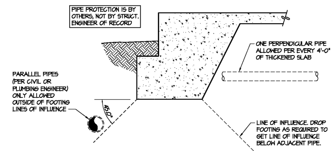
1 SECTION AT UNDERGROUND PIPE NOT TO SCALE
