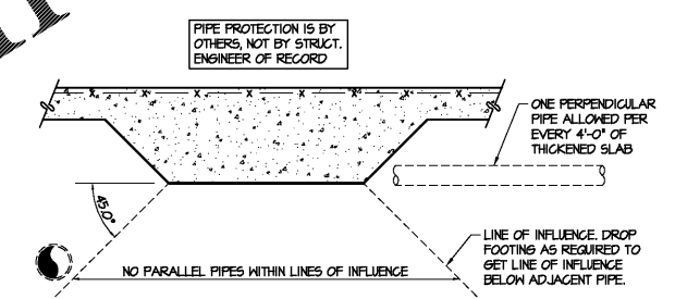
2 SECTION AT UNDERGROUND PIPE NOT TO SCALE
