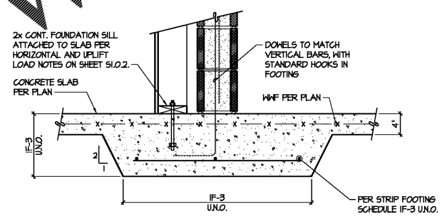
5 SECTION AT CMU WALL NOT TO SCALE
