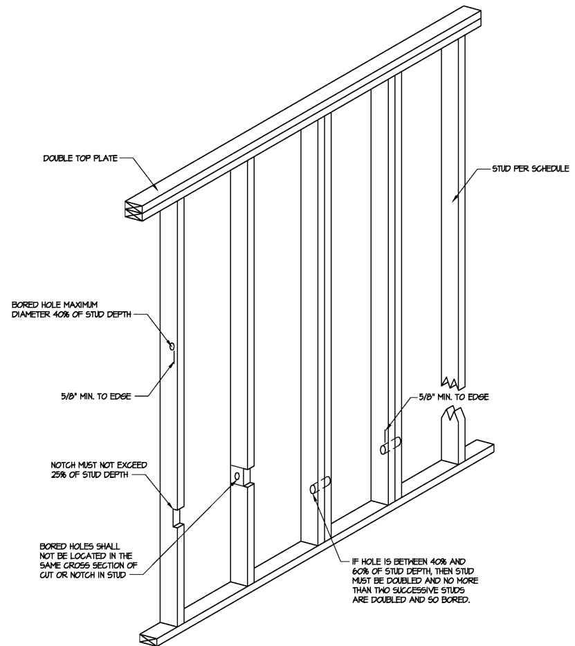
1 ALLOWABLE BEARING STUD PENETRATIONS NOT TO SCALE
