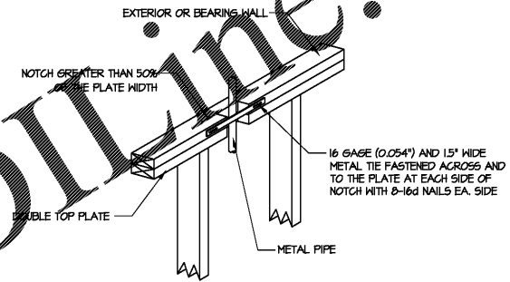
2 ALLOWABLE TOP PLATE PENETRATIONS NOT TO SCALE
