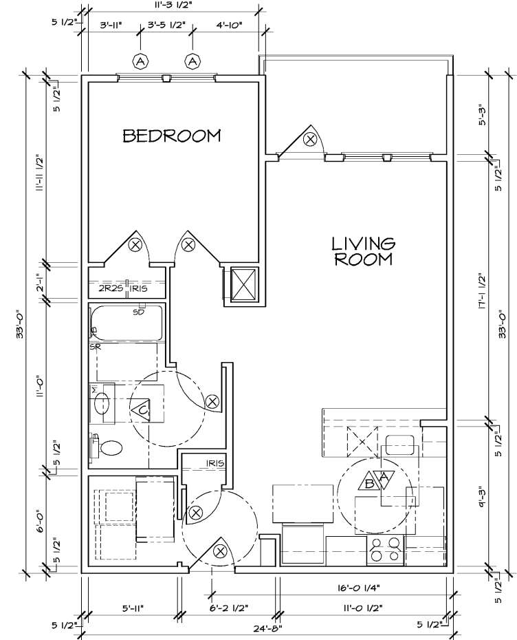
2 HC UNIT TYPE B1 - FLOOR PLAN A2.06 741 HEATED SQ FT / 838 GROSS SQ FT I.B.C. TYPE 'A' H.C. UNIT - UNIT #s 17, 59 & 95 1/4"=1'-0"
