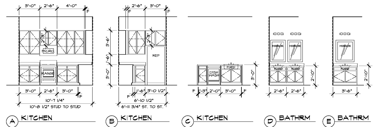
UNIT TYPE D1 - INTERIOR ELEVATIONS
