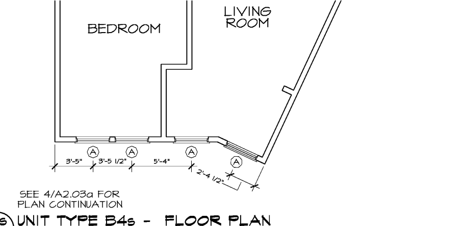
4s UNIT TYPE B4s - FLOOR PLAN A2.03a 926 HEATED SQ FT / 926 GROSS SQ FT I.B.C. TYPE 'B' H.C. UNIT 1/4"=1'-0"
