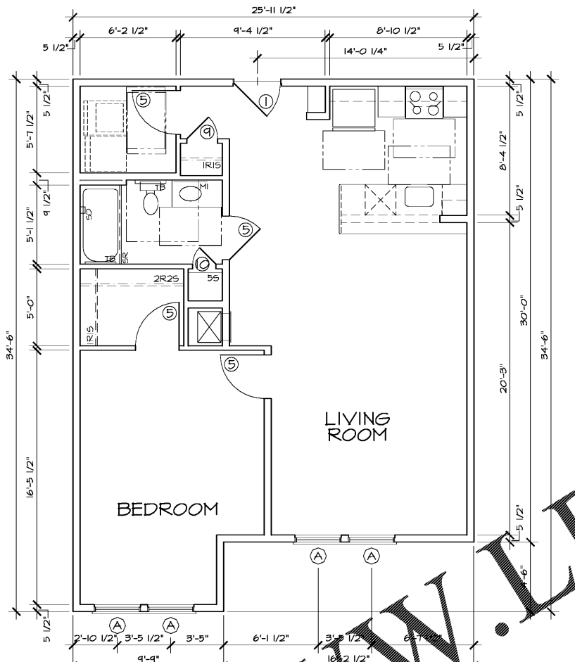
5 UNIT TYPE B5 - FLOOR PLAN A2.03a 816 HEATED SQ FT / 816 GROSS SQ FT I.B.C. TYPE 'B' H.C. UNIT 1/4"=1'-0"
