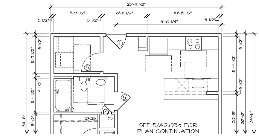
5a UNIT TYPE B5a - FLOOR PLAN A2.03a 816 HEATED SQ FT / 816 GROSS SQ FT I.B.C. TYPE 'B' H.C. UNIT 1/4"=1'-0"
