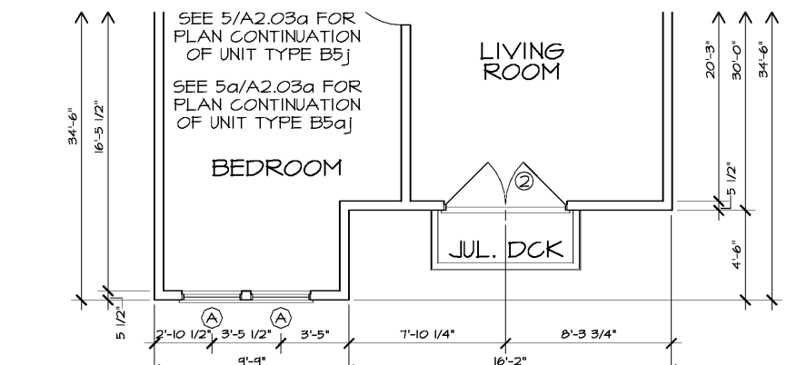
5j UNIT TYPE B5j / B5aj - FLOOR PLAN A2.03a 816 HEATED SQ FT / 834 GROSS SQ FT I.B.C. TYPE 'B' H.C. UNIT 1/4"=1'-0"
