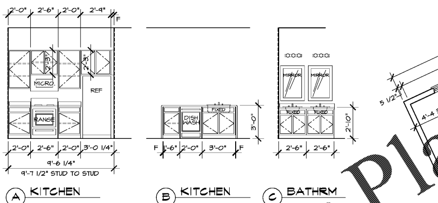
UNIT TYPES B6/B6j - INT. ELEVATIONS SEE SHEET A2.03 FOR INTERIOR ELEVATIONS FOR UNIT TYPES B4 & B5
