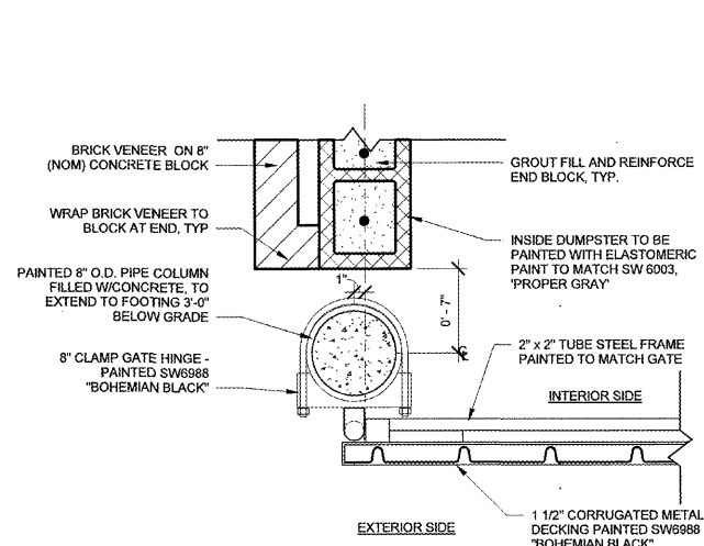
4 DUMPSTER GATE DETAIL A-402 SCALE: 1 1/2" = 1'-0"
