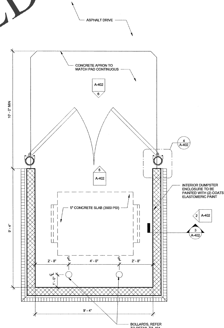
1 DUMPSTER ENCLOSURE PLAN A-402 SCALE: 1/2" = 1'-0"
