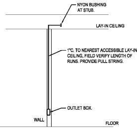
3 CATV WALL OUTLET DETAIL SCALE: NONE
