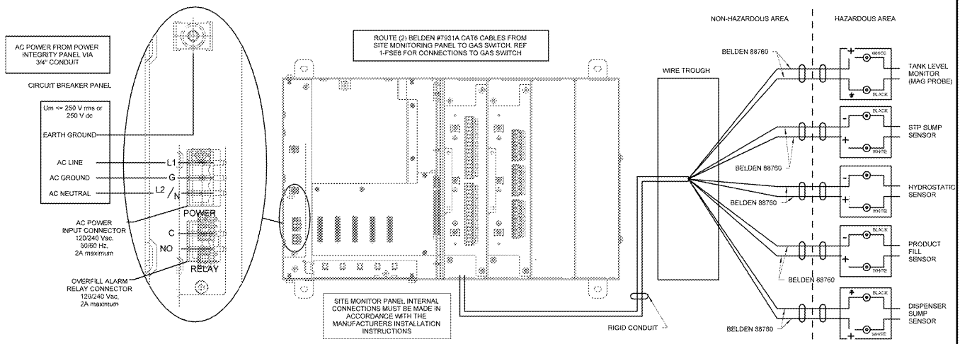
1 VEEDER-ROOT CONSOLE (SITE MONITOR PANEL) NTS
