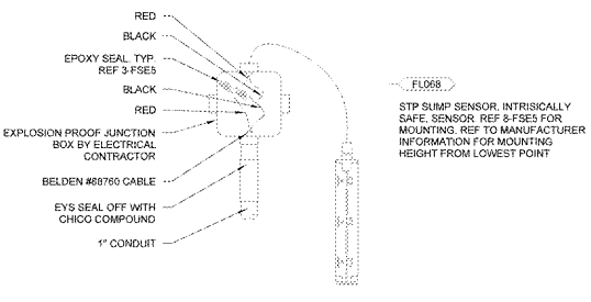
4 STP SUMP SENSOR MOUNTING DETAIL NTS
