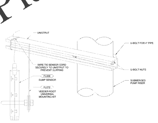
2 SPLIT TANK SENSOR SUPPORT NTS
