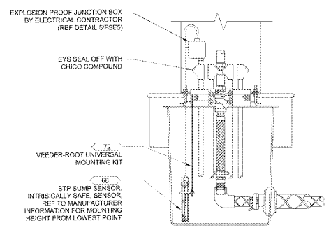
6 STP SUMP SENSOR MOUNTING DETAIL NTS
