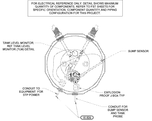
4 STP SUMP SECTION (TYPICAL) NTS
