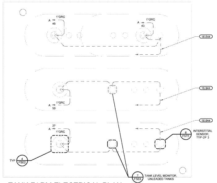
1 TANK FARM ELECTRICAL PLAN 3/32" = 1'-0"
