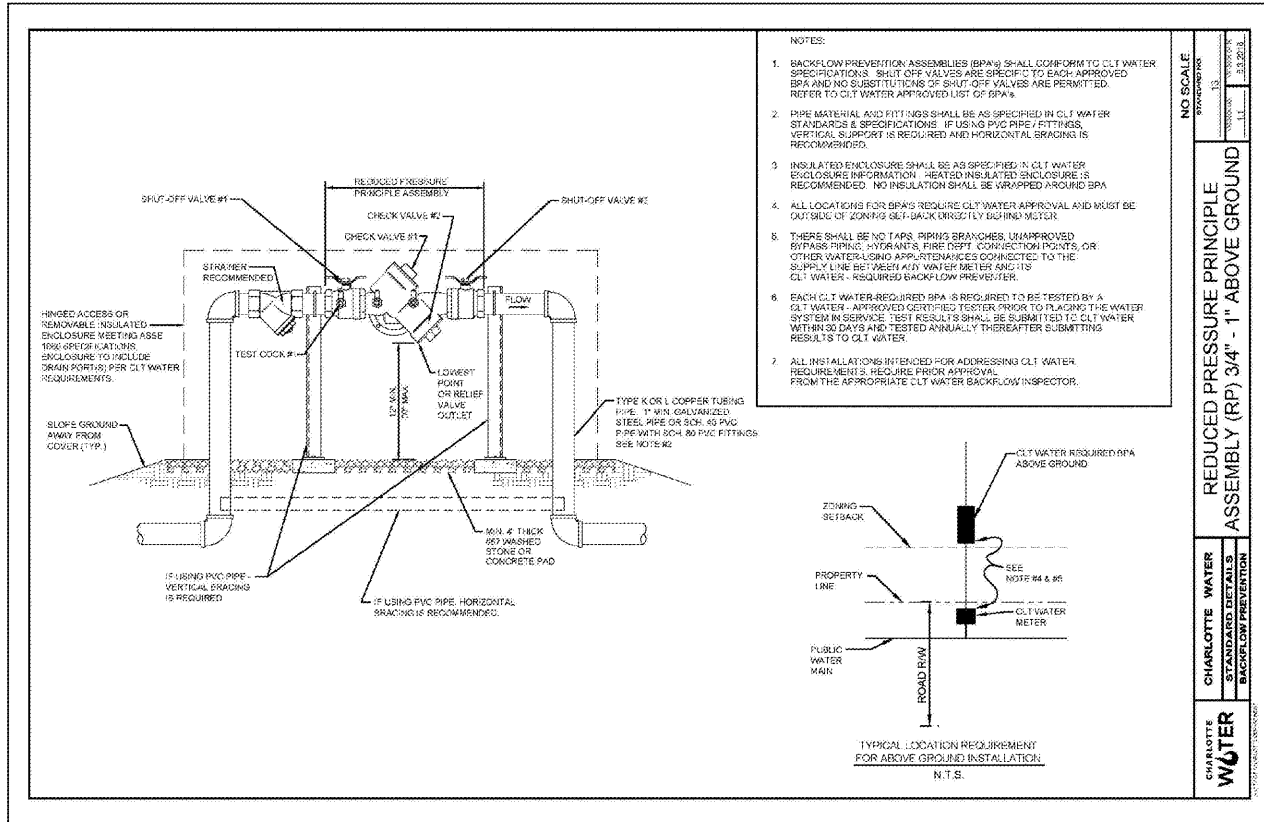
BACKFLOW PREVENTER
