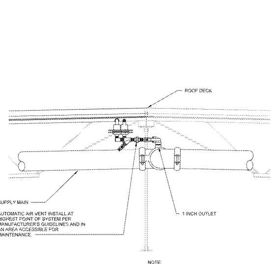
1 AIR RELEASE VENT NTS
