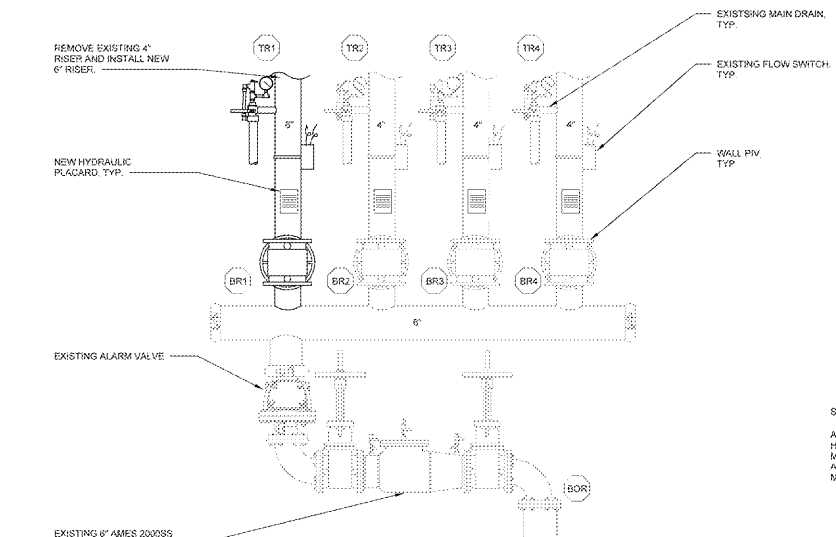
2 SPRINKLER RISER NTS
