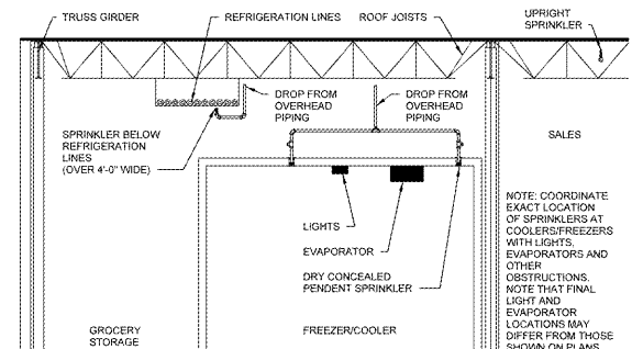
4 FREEZER SECTION NTS
