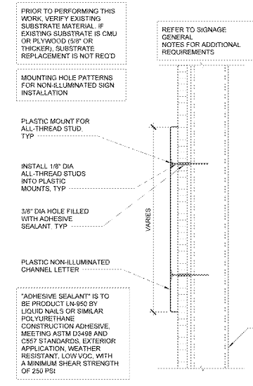
12 SIGN ATTACHMENT AT EIFS AND METAL STUD WALL 1 1/2" x 1-0"
