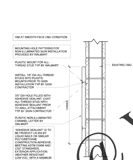
11 SIGN ATTACHMENT AT CMU WALL 1 1/2" x 1-0"
