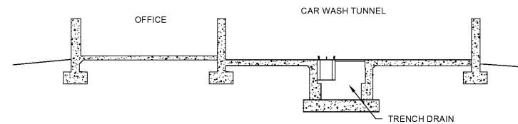
TRENCH DRAIN SECTION
