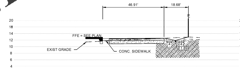
SECTION G-G
