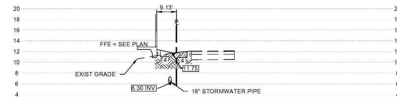
SECTION H-H
