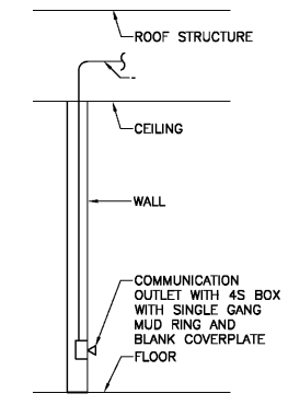
9 COMMUNICATION ROUGH-IN NO SCALE
