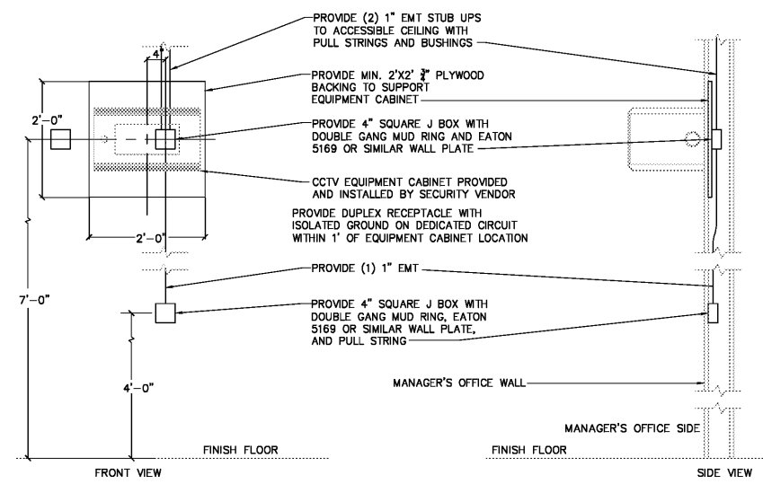
4 CCTV EQUIPMENT CABINET NO SCALE
