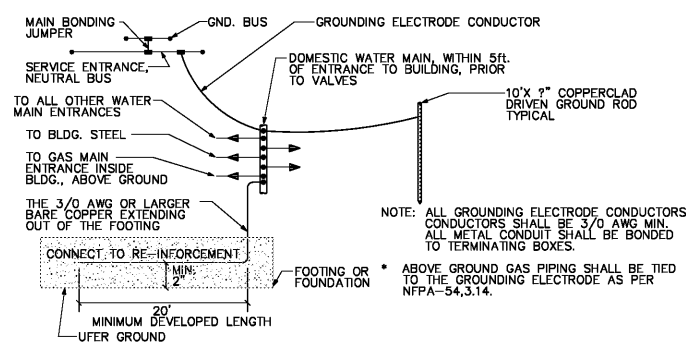
1 SERVICE ENTRANCE GROUNDING NO SCALE
