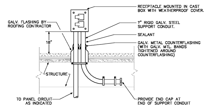
2 ROOF RECEPTACLE MOUNTING NO SCALE
