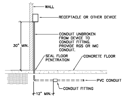
8 SERVICE AREA CONDUIT TRANSITION NO SCALE
