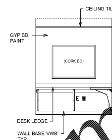
4 MANAGERS OFFICE - NORTH SEE ROOM FINISH SCHEDULE FOR FINISHES 1/4" = 1'-0"
