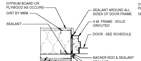
2 DOOR JAMB DETAIL A6 SCALE: 1 1/2"=1'-0"
