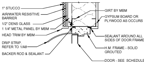
1 DOOR HEAD DETAIL A6 SCALE: 1 1/2"=1'-0"
