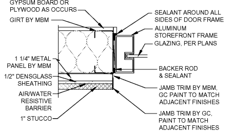
6 WINDOW JAMB DETAIL A6 SCALE: 1 1/2"=1'-0"
