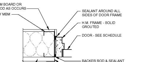
3 DOOR JAMB DETAIL A6 SCALE: 1 1/2"=1'-0"
