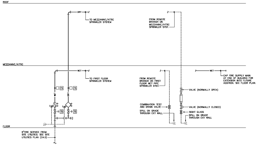
SPRINKLER SYSTEM SCHEMATIC DIAGRAM NO SCALE
