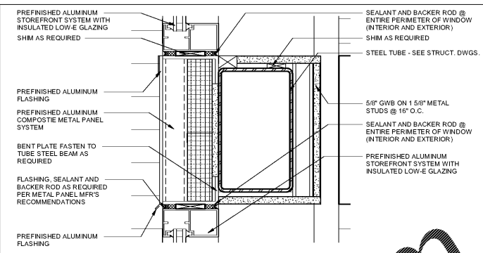
WALL SECTION DETAIL 3'-1'-0" 3
