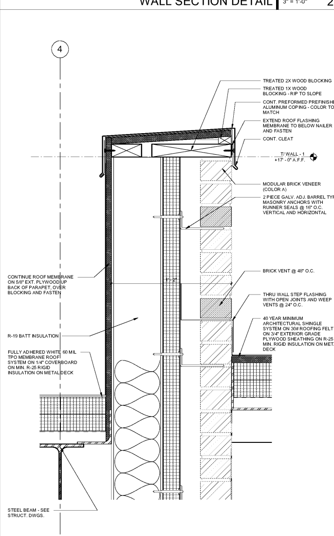
WALL SECTION DETAIL 3'-1'-0" 1
