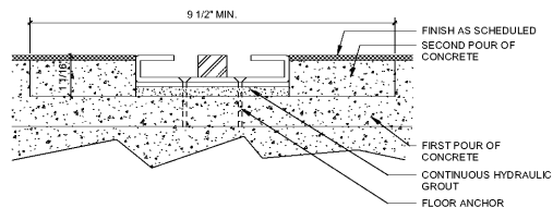
RECESSED RAIL DETAIL (ALTERNATE #2) 6'-1'-0" 6
