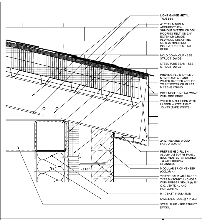
WALL SECTION DETAIL 3" = 1'-0" 5
