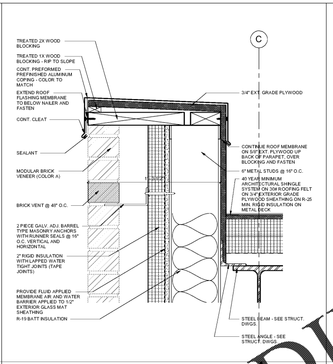
WALL SECTION DETAIL 3" = 1'-0" 4
