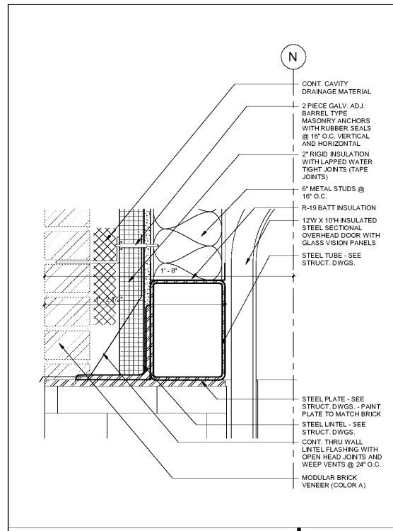
WALL SECTION DETAIL 3" = 1'-0" 6
