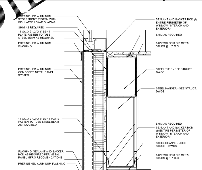
WALL SECTION DETAIL 3" = 1'-0" 3
