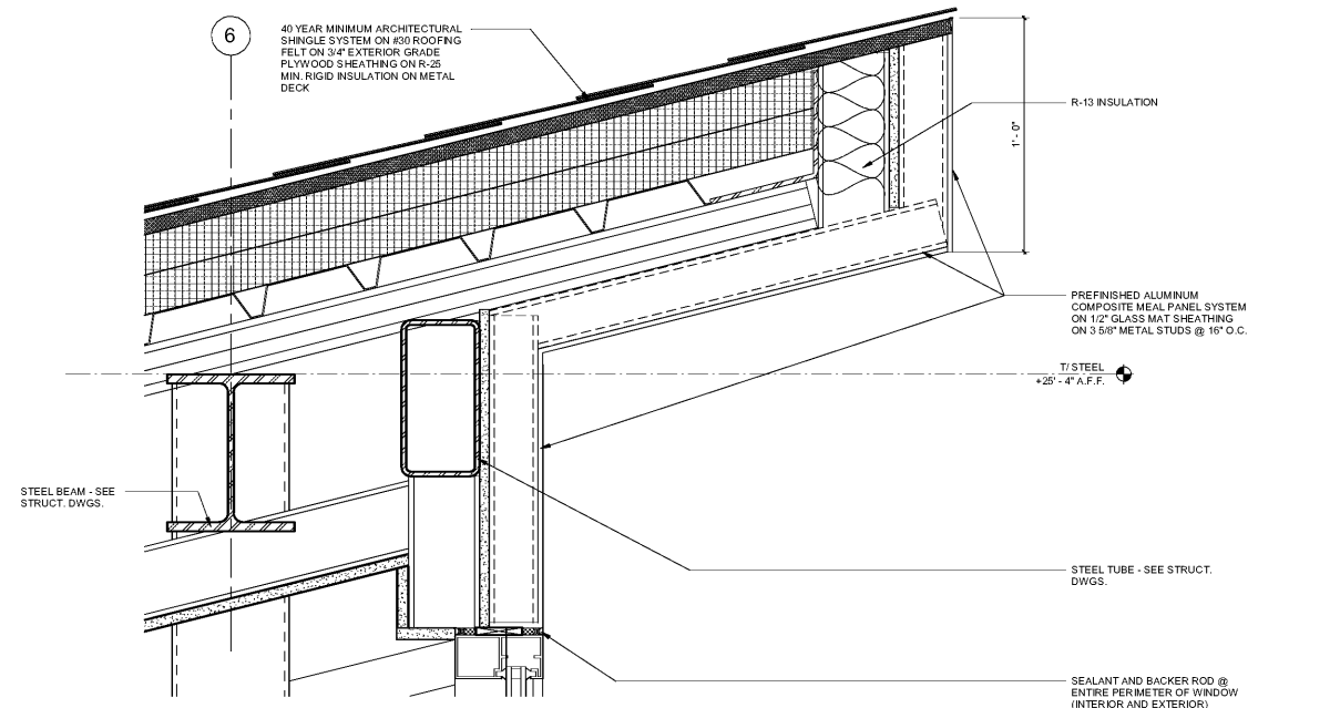
WALL SECTION DETAIL 3" = 1'-0" 6
