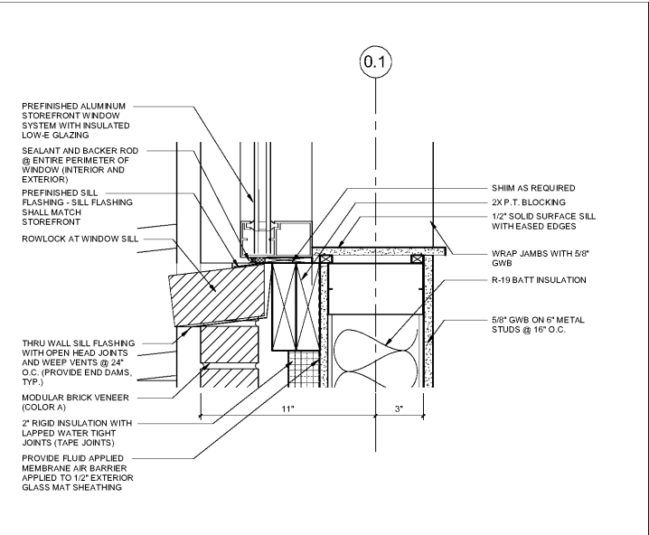
WALL SECTION DETAIL 3" = 1'-0" 8
