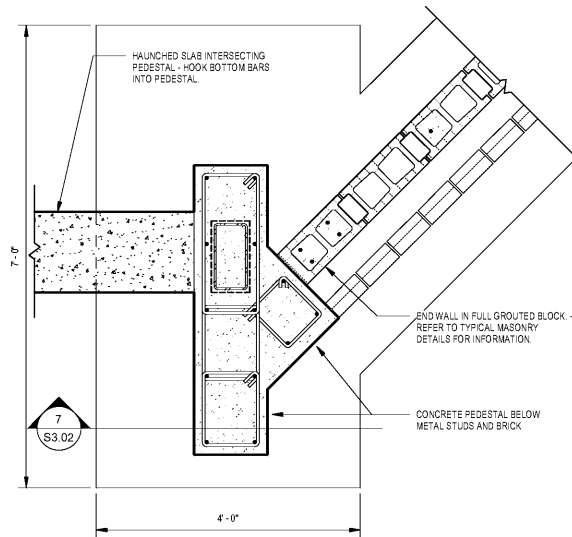
6 DETAIL - FOUNDATION S3.02 3/4" = 1'-0"
