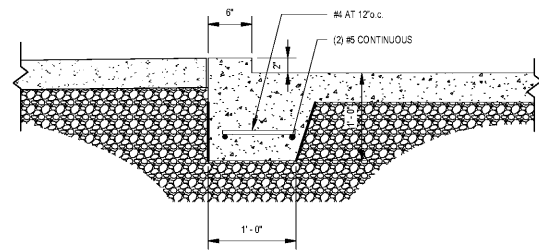
8 DETAIL - FOUNDATION S3.02 1" = 1'-0"
