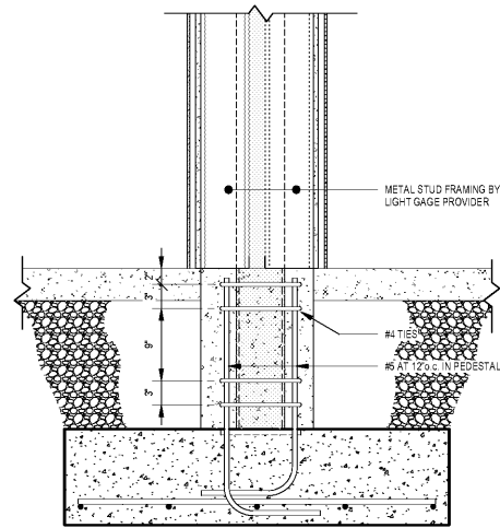
7 DETAIL - FOUNDATION S3.02 1" = 1'-0"
