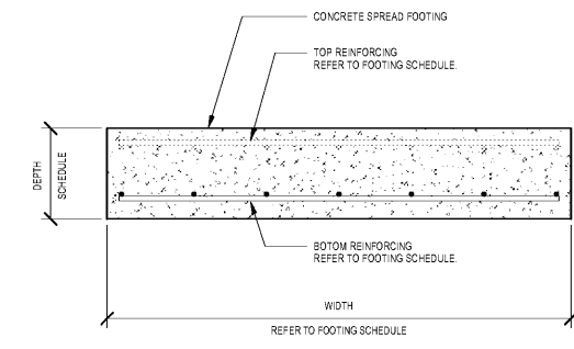
1 SPREAD FOOTING DETAIL - TYPICAL S3.01 3/4" = 1'-0"
