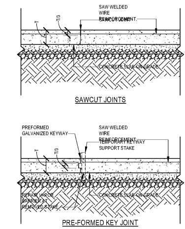
2 SLAB JOINT DETAIL - TYPICAL S3.01 1" = 1'-0"
