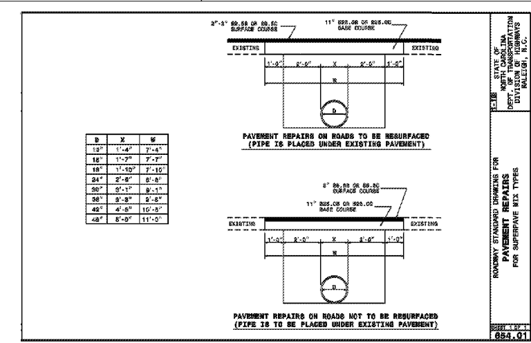
8 / C801 NCDOT PAVEMENT REPAIR NTS
