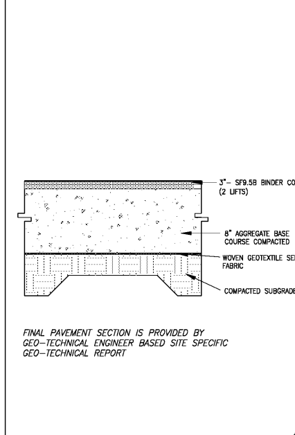
3 / C801 HEAVY DUTY ASPHALT PAVING NTS
