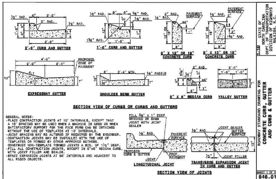
1 / C801 NCDOT CURB AND GUTTER NTS
