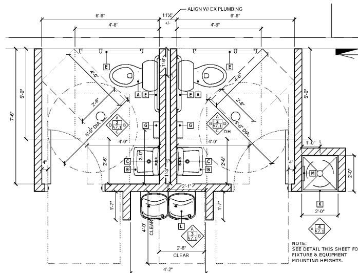
1 ENLARGED TOILET PLAN SCALE: 1/2" = 1'-0"
