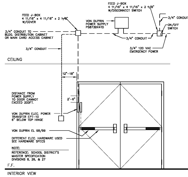
1 CARD ACCESS DETAIL FOR SCHOOL DISTRICT ES.15
