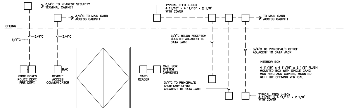
3 TYPICAL MAIN ENTRANCE ES.15
