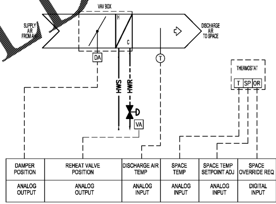
2 VAV BOX CONTROL SCHEMATIC TYPICAL OF ALL VAVs
