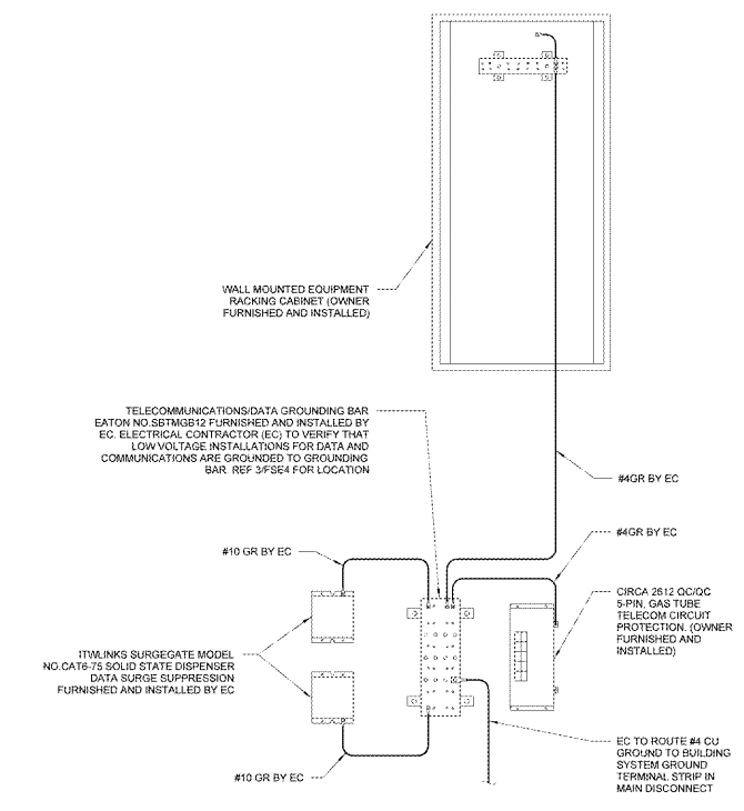
5 LOW VOLTAGE GROUNDING SCHEMATIC NTS
