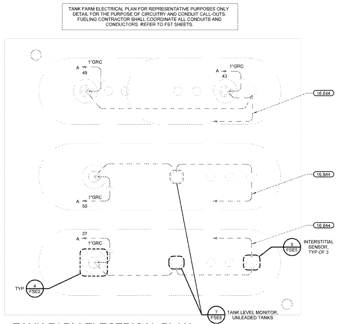
1 TANK FARM ELECTRICAL PLAN 3/32" = 1'-0"
