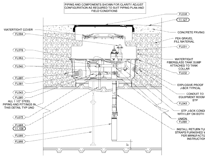
8 DIESEL STP SUMP SECTION NTS
