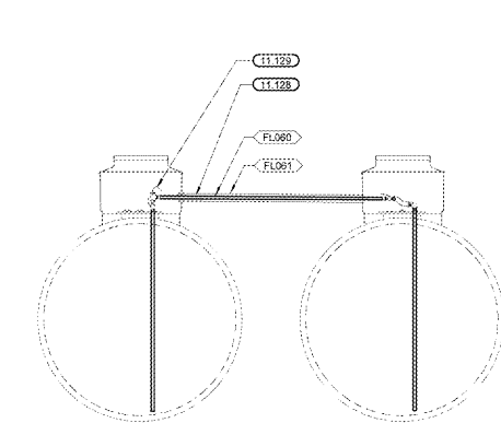
9 EQUALIZATION PIPING SECTION NTS
