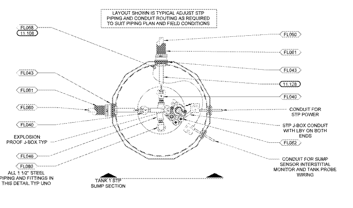
1 UNLEADED STP SUMP PLAN TANK #1 NTS
