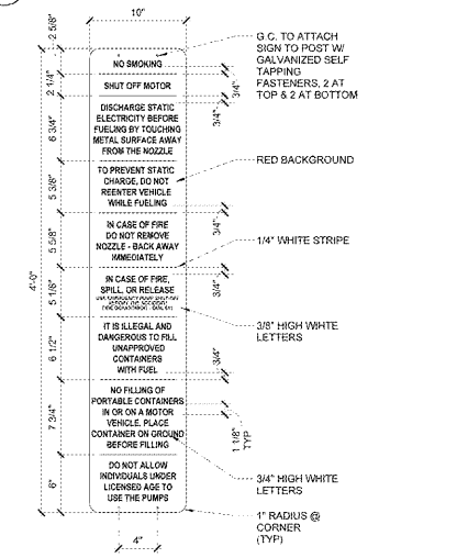
1 SIGNAGE @ COLUMNS 1 1/2' x 1'-0"
