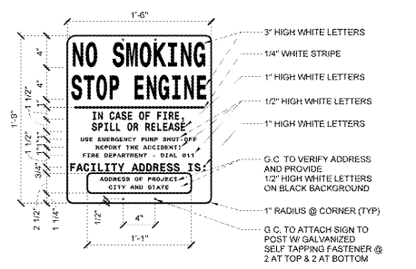
2 SIGNAGE @ TELEPHONE POST 1 1/2' x 1'-0"
