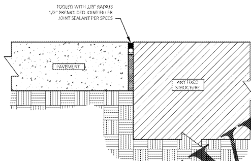
ISOLATION JOINT
