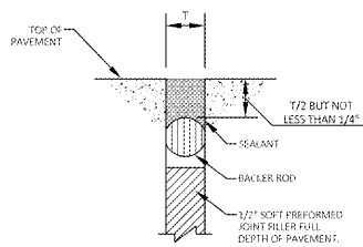
BACKER ROD AND SEALANT SECTION AT FIXED STRUCTURE
