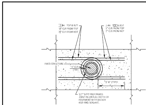
TYPICAL ROUND FIXED STRUCTURE PLAN DETAIL USES: MANHOLES, LIGHT POLE BASES AND BOLLARDS
