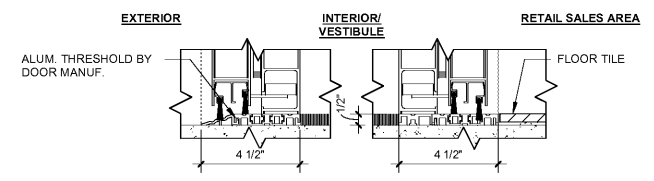
8 TRANSITION DETAIL @ VESTIBULE DOOR 3" = 1'-0"
