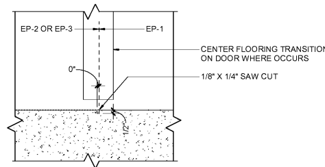
5 TS-5 SECTION DETAIL 3" = 1'-0"
