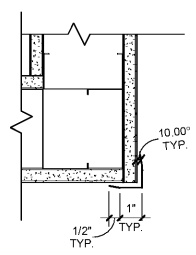
6 CG-1 PLAN DETAIL 3" = 1'-0"
