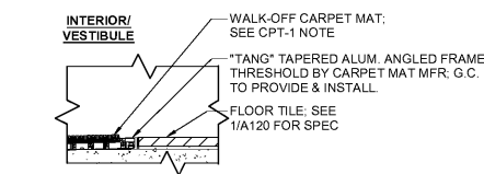
9 TRANSITION DETAIL @ VESTIBULE TILE 3" = 1'-0"
