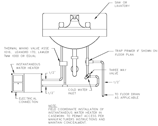
INSTANTANEOUS WATER HEATER NO SCALE
