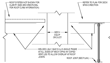
6 MECHANICAL ROOF FRAME OPENING 1 1/2" x 1-0"
