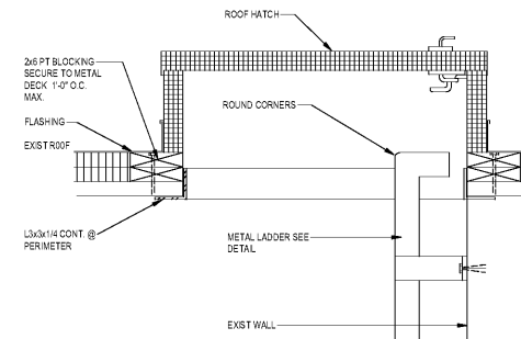
3 MEMBRANE ROOF HATCH 1 1/2" x 1-0"
