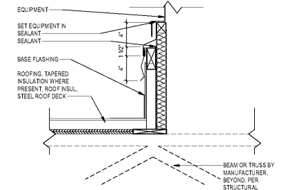
4 MANUFACTURED CURB FLASHING 1 1/2" x 1-0"
