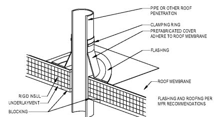
2 MEMBRANE PIPE FLASHING 1 1/2" x 1-0"
