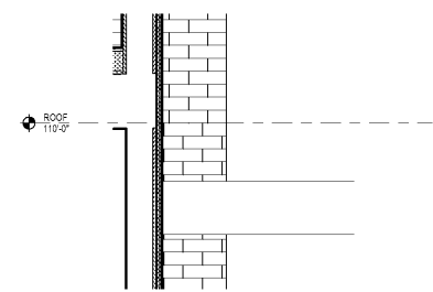
3 SECTION DETAIL 3/16" = 1'-0"
