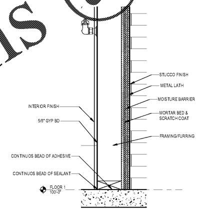
2 EXTERIOR WOOD FRAME WALL 1/12" = 1'-0"
