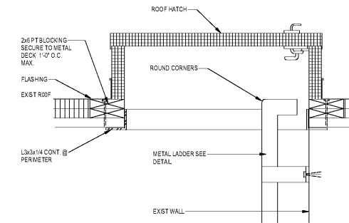
MEMBRANE ROOF HATCH 1 1/2" x 1 1/2"
