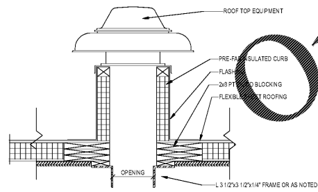
MEMBRANE EQUIPMENT CURB 1 1/2" x 1 1/2"
