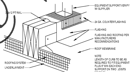
MEMBRANE EQUIPMENT SUPPORT 1 1/2" x 1 1/2"
