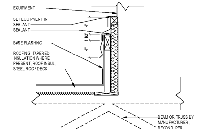
MANUFACTURED CURB FLASHING 1 1/2" x 1 1/2"
