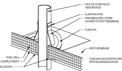
MEMBRANE PIPE FLASHING 1 1/2" x 1 1/2"
