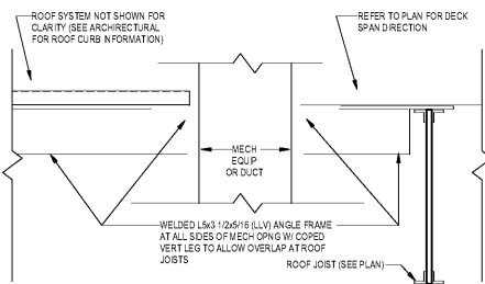
MECHANICAL ROOF FRAME OPENING 1 1/2" x 1 1/2"
