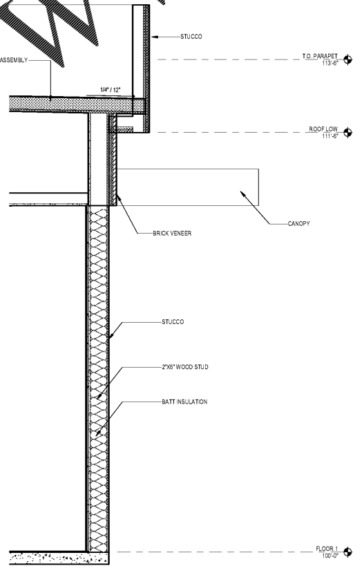
1 WALL SECTION 3/4" = 1'-0"
