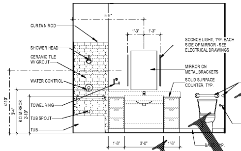
9 A1A-BATHROOM ELEVATION - WEST
