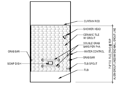
8 A1A- BATHROOM ELEVATION - SOUTH
