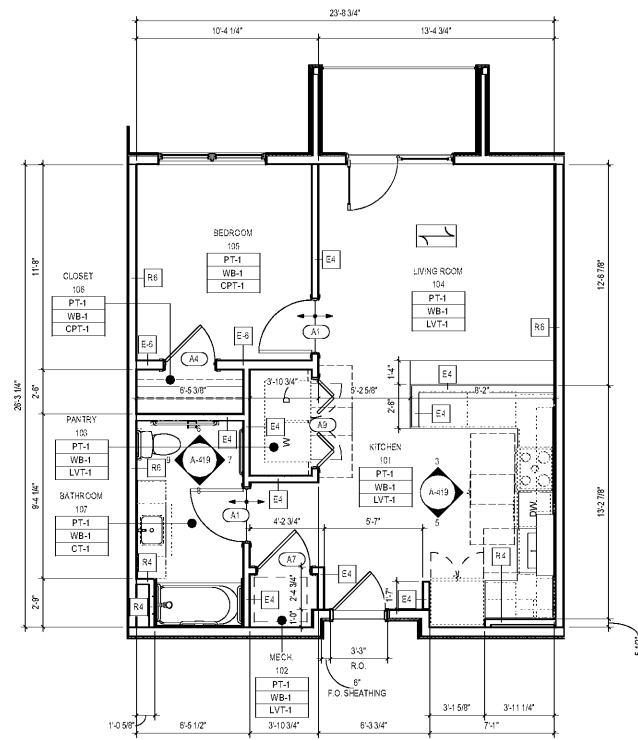
1 UNIT PLAN - A1A 1-BEDROOM
