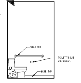
6 A1A- BATHROOM ELEVATION - NORTH
