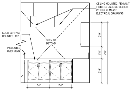
3 A1A- KITCHEN ELEVATION - NORTH
