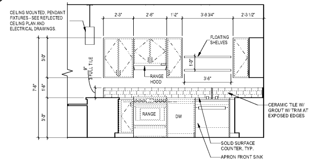
4 A1A- KITCHEN ELEVATION - EAST
