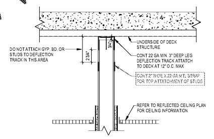
1 (30x42) NON-RATED - PERPENDICULAR TO FLUTES 1:1/2" x 1'-0"
