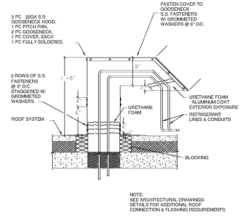
07M111 REFRIGERANT ROOF PENETRATION NO SCALE
