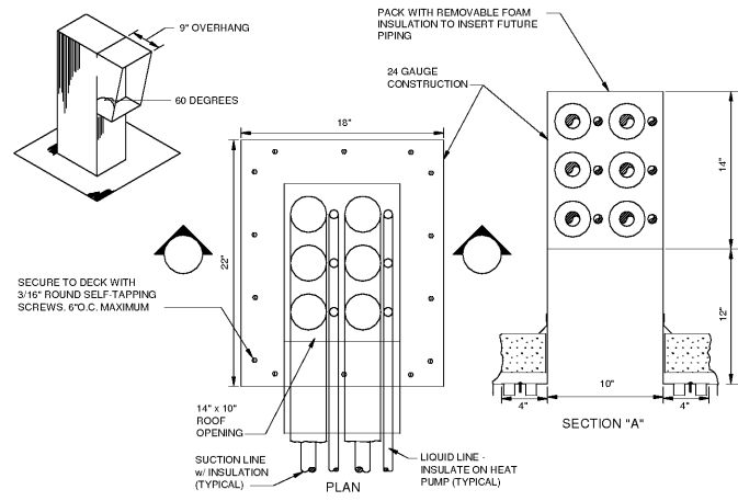
07M101 REFRIGERANT PIPE CURB NO SCALE
