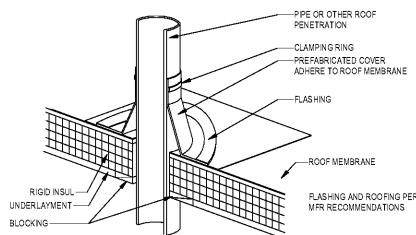
3 MEMBRANE PIPE FLASHING 1 1/2" x 1-0"
