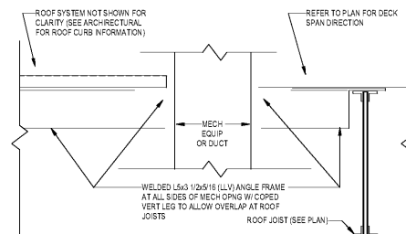
2 MECHANICAL ROOF FRAME OPENING 1 1/2" x 1-0"
