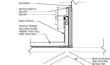
5 MANUFACTURED CURB FLASHING 1 1/2" x 1-0"
