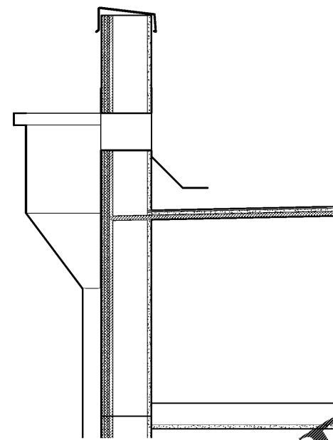
8 CONDUCTOR HEAD DETAIL 1 1/2" x 1-0"
