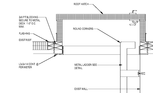
1 MEMBRANE ROOF HATCH 1 1/2" x 1-0"
