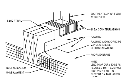
6 MEMBRANE EQUIPMENT SUPPORT 1 1/2" x 1-0"
