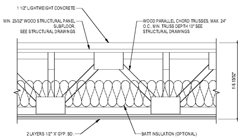
3 1 HOUR STC 55 TRUSS FLOOR ASSEMBLY (LWC) 1 1/2" x 12"
