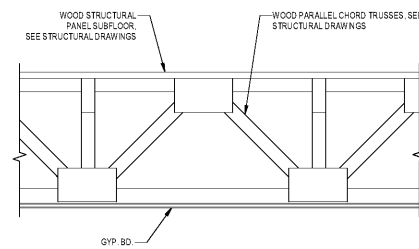
2 NON-RATED TRUSS FLOOR ASSEMBLY 1 1/2" x 12"
