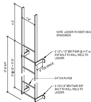
1 STAIRS WALL LADDER 3/4" x 17"
