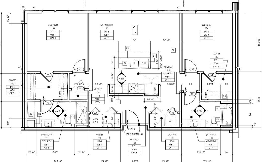
1 UNIT PLAN - B4 2-BEDROOM 14' x 11'-0"
