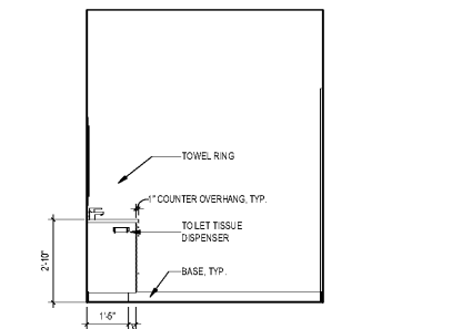
8 BATHROOM ELEVATION - WEST 38" x 1'-0"
