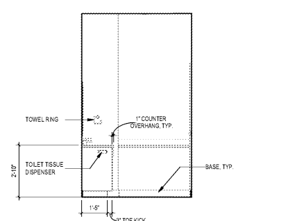
12 BATHROOM 2 ELEVATION - WEST 38" x 1'-0"
