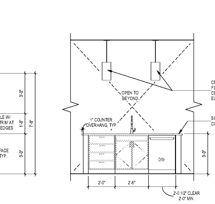
3 KITCHEN ELEVATION - NORTH 38" x 1'-0"
