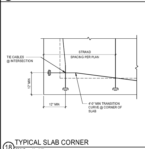
18 TYPICAL SLAB CORNER SCALE: 1" = 1'-0"
