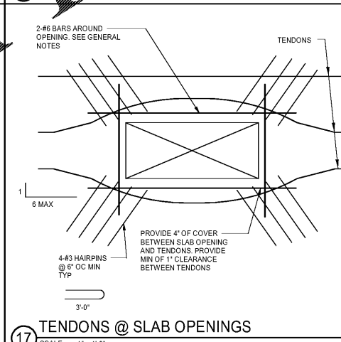
17 TENDONS @ SLAB OPENINGS SCALE: 1" = 1'-0"
