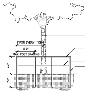
5 TREE PROTECTION BARRICADE SCALE - NTS
