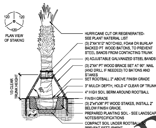
7 PALM STAKING: SABAL PALM SCALE - NTS
