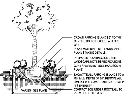
4 PARKING ISLAND PLANTING SCALE - NTS
