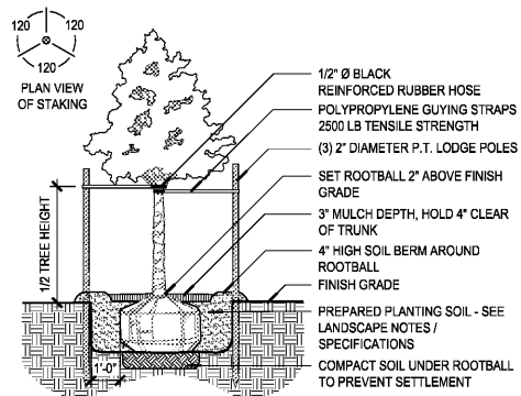
1 TREE STAKING: <3" CALIPER SCALE - NTS
