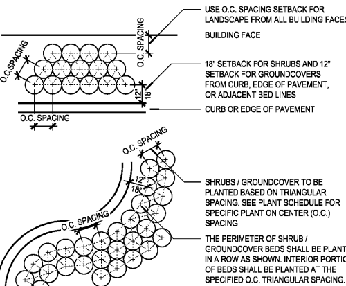
9 SHRUB / GROUND COVER SPACING SCALE - NTS
