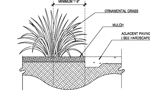
11 ORNAMENTAL GRASS PLANTING DETAIL SCALE - NTS
