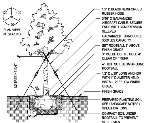
2 TREE STAKING: 3"-7" CALIPER - CABLE SCALE - NTS
