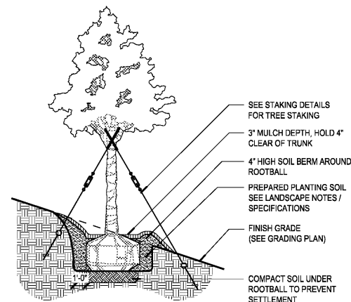
3 TREE PLANTING ON SLOPE SCALE - NTS
