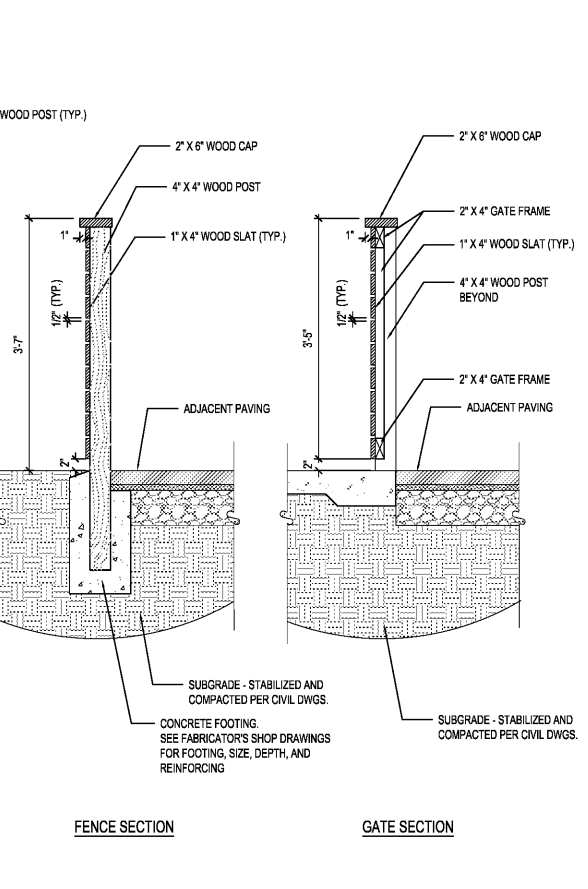
5 F2 - WOOD FENCE & GATE SECTION SCALE: 1" = 1'-0"
