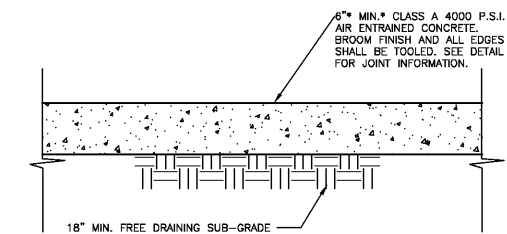
CONCRETE SECTION SEE GEOTECHNICAL REPORT FOR ADDITIONAL INFORMATION ** CONCRETE FOR ALL SIDEWALKS NOT SUBJECT TO VEHICLE TRAFFIC
