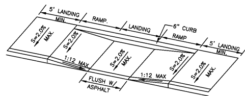
PARALLEL SIDEWALK RAMP DETAIL N.T.S.
