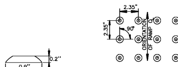
TRUNCATED DOMES DETAIL N.T.S.
