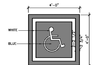
PAINTED ACCESSIBLE SYMBOL N.T.S. *MARKING TO BE PER FDOT INDEX 17346
