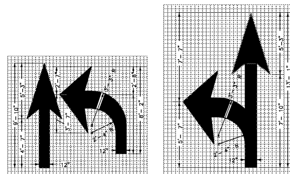
DIRECTIONAL & TURN ARROW DETAIL N.T.S.
