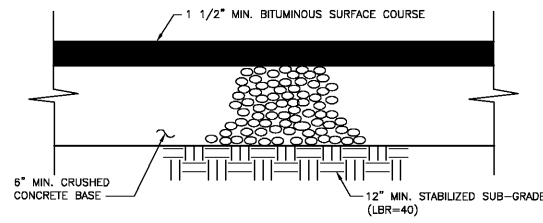
STANDARD DUTY PAVEMENT SECTION SEE GEOTECHNICAL REPORT FOR ADDITIONAL INFORMATION
