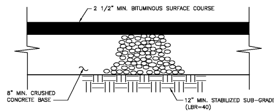
HEAVY DUTY PAVEMENT SECTION SEE GEOTECHNICAL REPORT FOR ADDITIONAL INFORMATION
