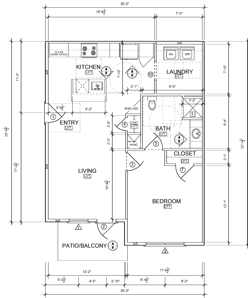
1 UNIT A-1a FLOOR PLAN - HC A3.11 SCALE 1/4"=1'
